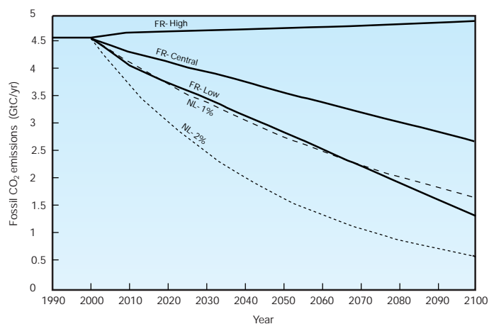
Figure B2. Fossil CO 2 emissions (GtC/yr) for Annex I countries under the French (FR) and Netherlands (NL) emissions limitation proposals. FR-High, FR-Central and FR-Low are as shown in Figure B1. NL-1% and NL-2% correspond to 1 per cent and 2 per cent per year compound emissions reductions from the 2000 level.
