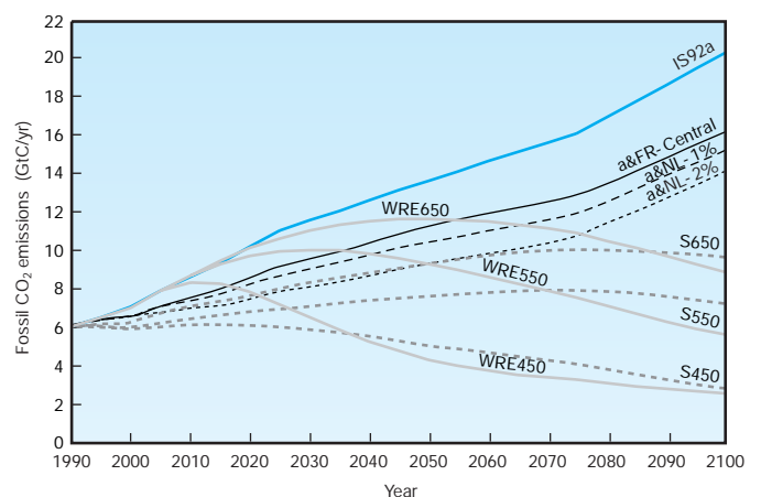
Figure 7. Global fossil CO 2 emissions (GtC/yr) for the IS92a scenario and modifications of it based on proposed limitations to Annex I country emissions (NL-1%, NL-2% and FR-Central) compared with emissions required to follow the S450, 550 and 650 and WRE450, 550 and 650 concentration stabilization profiles. Stabilization results calculated using the Bern model.
